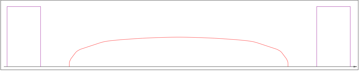
FIGURE 17. The barrier constructed in Proposition 7.3.
