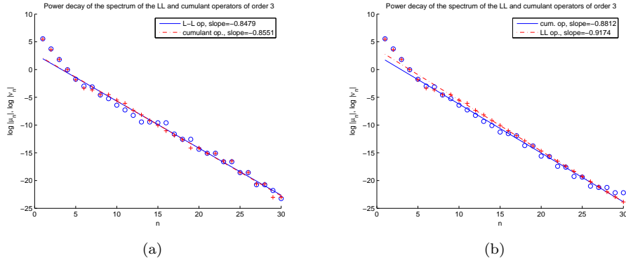
FIGURE 12. Exponential decay of the Spectrum of the cumulant operator \tilde{\mathcal{K}}_3 (denoted by +) and Lindeberg–Lyapunov operator \mathcal{K}_3 (denoted by \circ ): (a) single precision, (b) double precision
