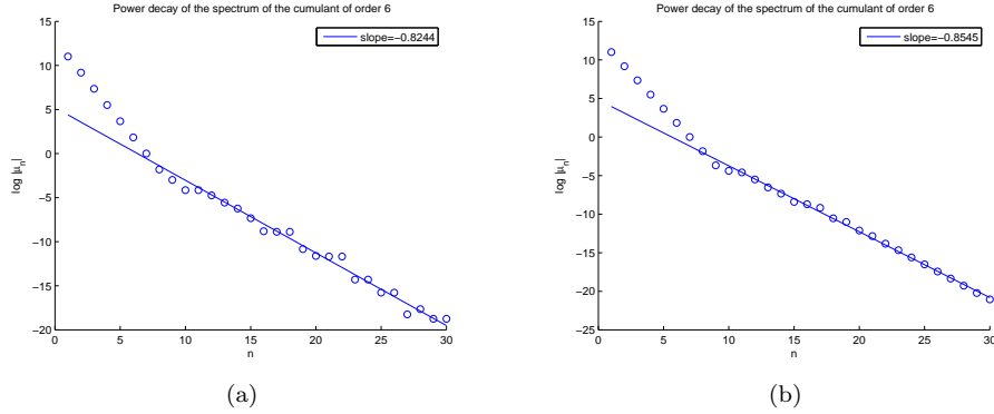
FIGURE 18. Exponential decay of the Spectrum of the cumulant operator \mathcal{K}_6 : (a) single precision, (b) double precision
