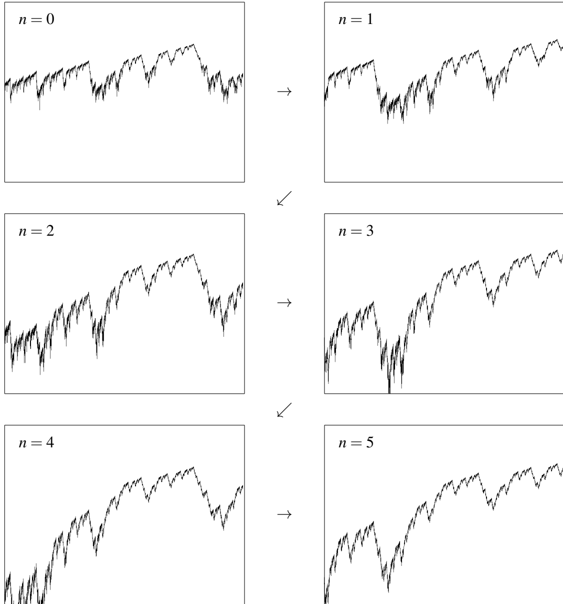
Figure 6: Consider zooms of \lambda(\theta) centered at \theta_0 = 1/6 with \lambda_0 = 1.521379707 . The width is 0.284 \times 2^{-n} and the height is 2.185 \times \lambda_0^{-n} . A left-sided maximum at \theta_0 was observed by Tan Lei and Thurston [21]. There seems to be a kind of self-similarity with respect to the combined scaling by 2^2 and by \lambda_0^2 , not by 2^1 and \lambda_0^1 . See Example 6.3 for the asymptotics of specific sequences; one of these shows that there is not a right-sided maximum at \theta_0 = 1/6 .
