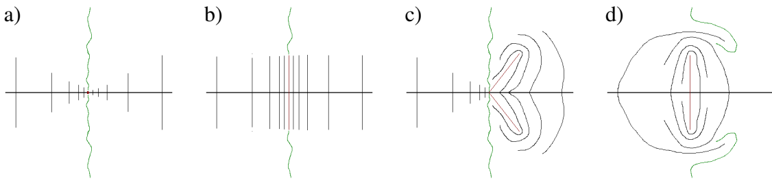
Figure 3: Possible scenarios at the Feigenbaum parameter c_F \in \mathcal{M} \cap \mathbb{R} : in a) \mathcal{M} is openly locally connected at c_F , and the fiber of c_F is non-trivial in the other cases [16, 47]. It is formed from the impressions of two rays. In case d) the rays do not land; they have non-trivial accumulation sets. This example could be modified, such that the impressions are larger than the accumulation sets. Note that in cases b) and d), \mathcal{M} \setminus \{c_F\} is not disconnected.
