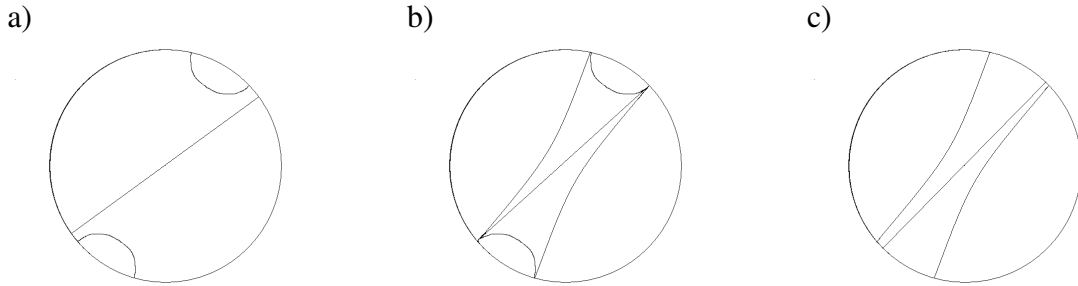
Figure 4: The pattern of rays landing together can be described by a lamination of the disk [56]. As \theta is varied, the diameter defined by \theta/2 and (\theta + 1)/2 is moving and disconnecting or reconnecting chords. The closed lamination is describing combinatorially biaccessing pairs of angles; the corresponding rays need not land together if \mathcal{K}_c is non-locally connected.
