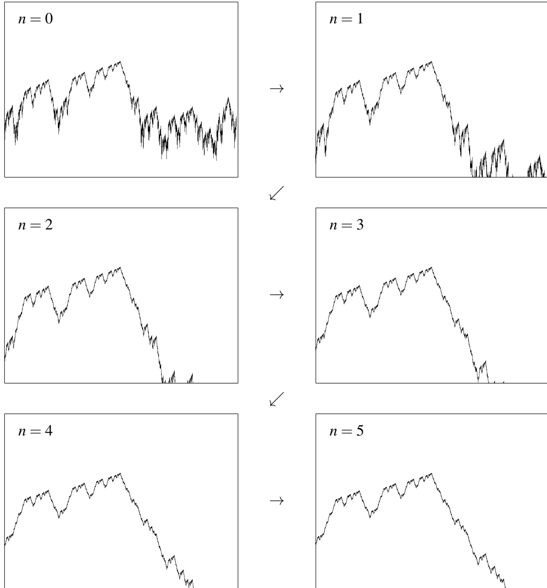
Figure 1: The biaccessibility dimension is related to the growth factor \lambda by B_{\text{comb}}(\theta) = \log(\lambda(\theta))/\log 2 . Consider zooms of \lambda(\theta) centered at \theta_0 = 1/4 with \lambda_0 = 1.69562077 . The width is 0.201 \times 2^{-n} and the height is 1.258 \times \lambda_0^{-n} . There seems to be a local maximum at \theta_0 and a kind of self-similarity with respect to the combined scaling by 2 and by \lambda_0 . See Example 6.1 for the asymptotics of B_{\text{comb}}(\theta) on specific sequences of angles \theta_n \rightarrow \theta_0 .
