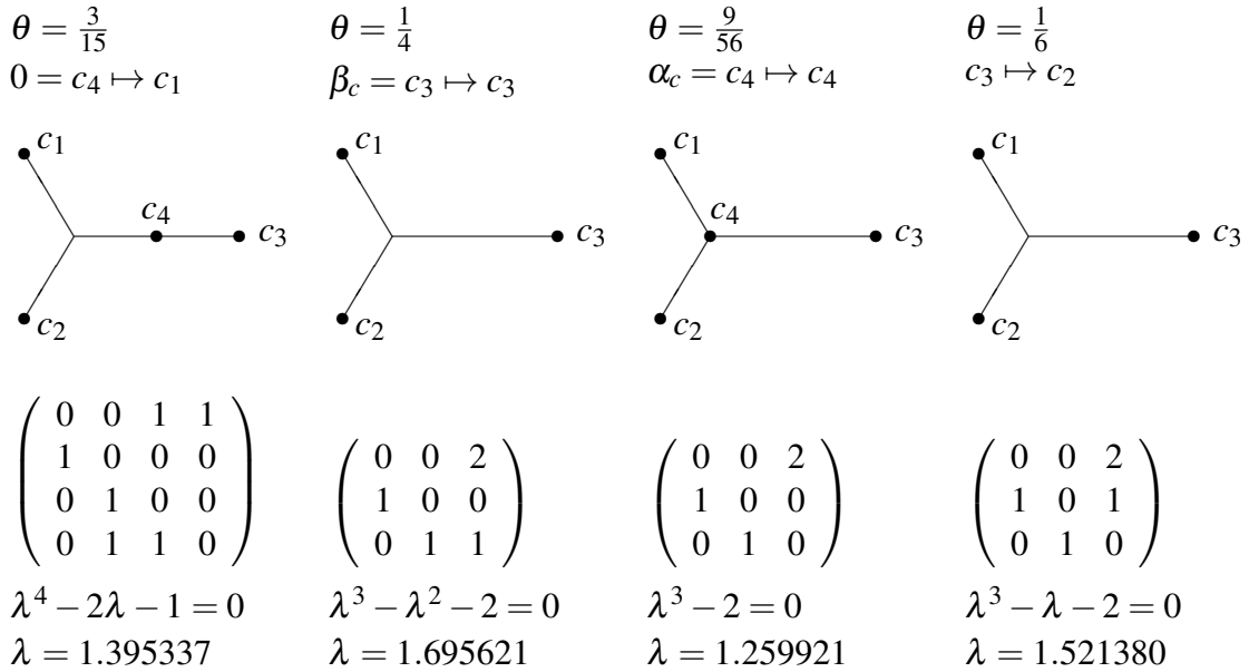
Figure 2: Examples of Hubbard trees and Markov matrices defined by an angle \theta . Here f_c(z) maps c = c_1 \mapsto c_2 \mapsto c_3 \mapsto c_4 and the edges are numbered such that the first edge is before c_1 = c .
