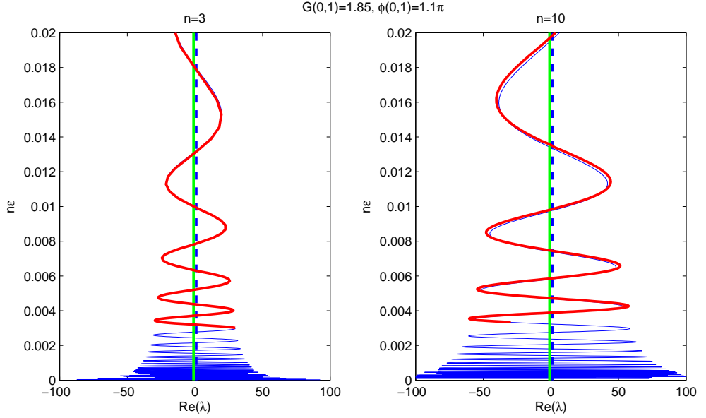
FIGURE 7. Oscillations of \Re(\lambda(\mu=0;\varepsilon)) at n=3, 10 . Thin line (blue) - analytical estimates (eq. (4.1)). Thick line (red) - numerical computations.
